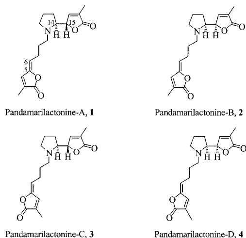
Figure 1. The Pandanus alkaloids
