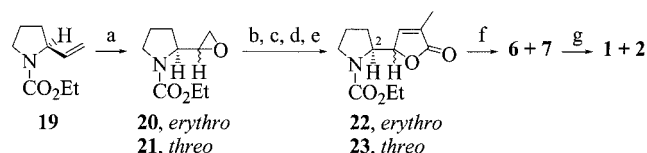
Scheme 3. Reagents and conditions: (a) MCPBA, CHCl 3 , room temp., 24 h, 77%; (b) separation of diastereoisomers; (c) PhSeCH(CH 3 )CO 2 H, LDA (2 equiv.), THF, 0 °C to room temp., 1.5 h; (d) AcOH, THF, reflux, 16 h; (e) H 2 O 2 , AcOH, 0 °C, 45 min, 61% from 20 ; (f) TMSI, CHCl 3 , reflux, 5 h, 84%; (g) 8 , pyridine, DMF, 60 °C, 3 days, 44%
