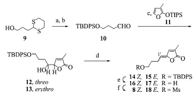
Scheme 1. Reagents and conditions: (a) TBDPSCl, Im, DMF, room temp., 96%; (b) CaCO 3 , MeI, CH 3 CN/H 2 O, room temp., 92%; (c) BF 3 ·Et 2 O, CH 2 Cl 2 , -78 °C, 2 h, 82%; (d) TMSCl, DBU, CHCl 3 , reflux, 1 h, 94%; (e) Bu 4 NF, THF, room temp., 3 h, 86%; (f) MsCl, pyridine, CH 2 Cl 2 , room temp., overnight, 74%
