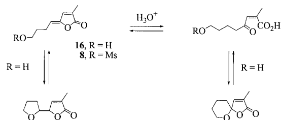
Scheme 2. Evolution pathways for lactones 8 and 16
