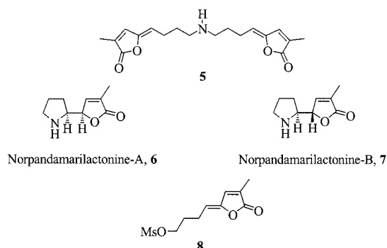
Figure 2. Synthetic precursors of pandamarilactonines
